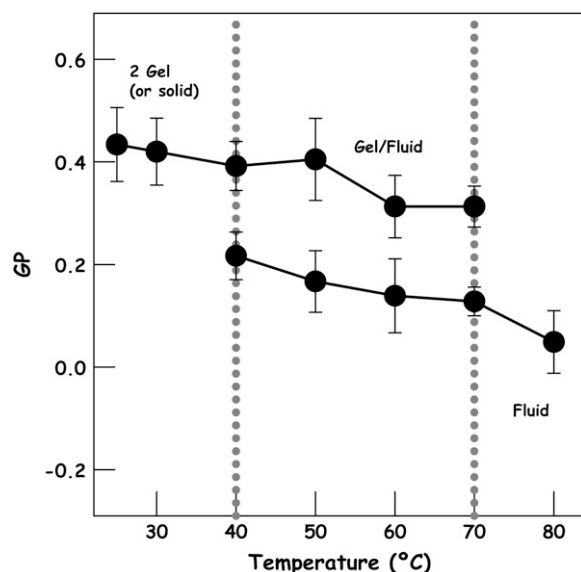
FIGURE 4 Laurdan GP average values of \text{HSC}(\text{Cer}/\text{Chol})/\text{FFA} at different temperatures. These values were obtained by analyzing eight different regions of each Laurdan GP image at the desired temperature. At least four different Laurdan GP images were analyzed per temperature. The dotted lines in the plot indicate the observed phase transition events in the microscopy experiments.
